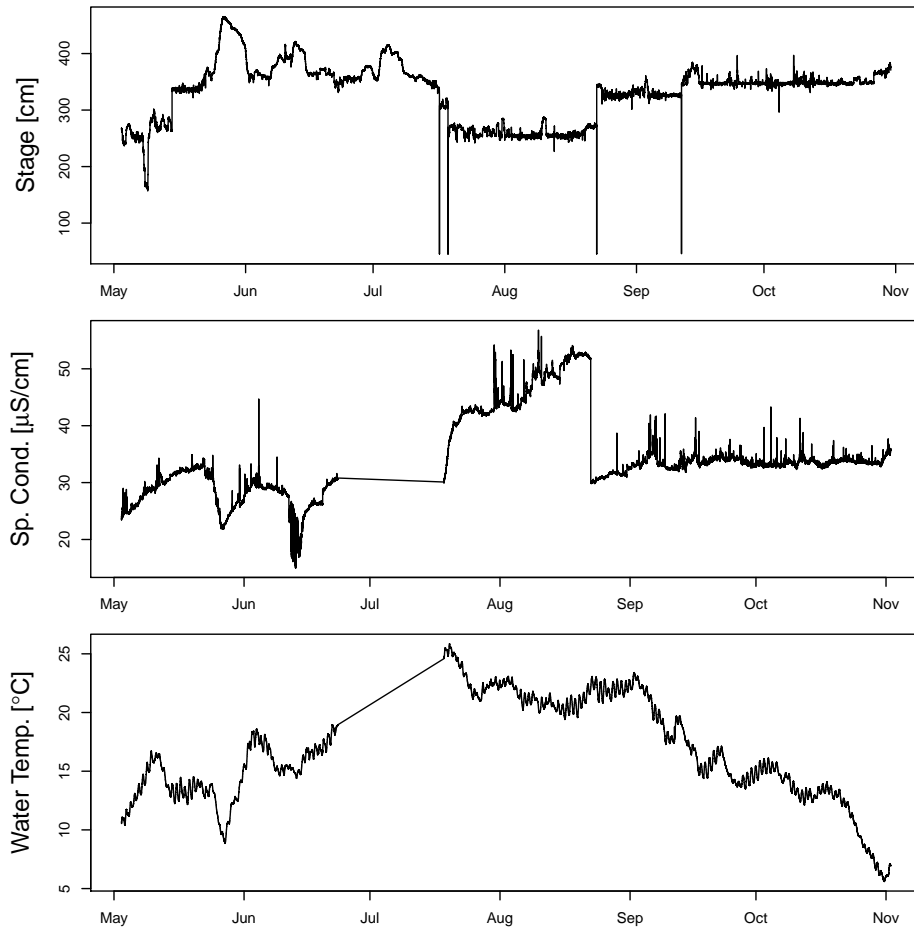
Figure 2: Stage, Specific Conductance and Water Temperature for ARD's full record
