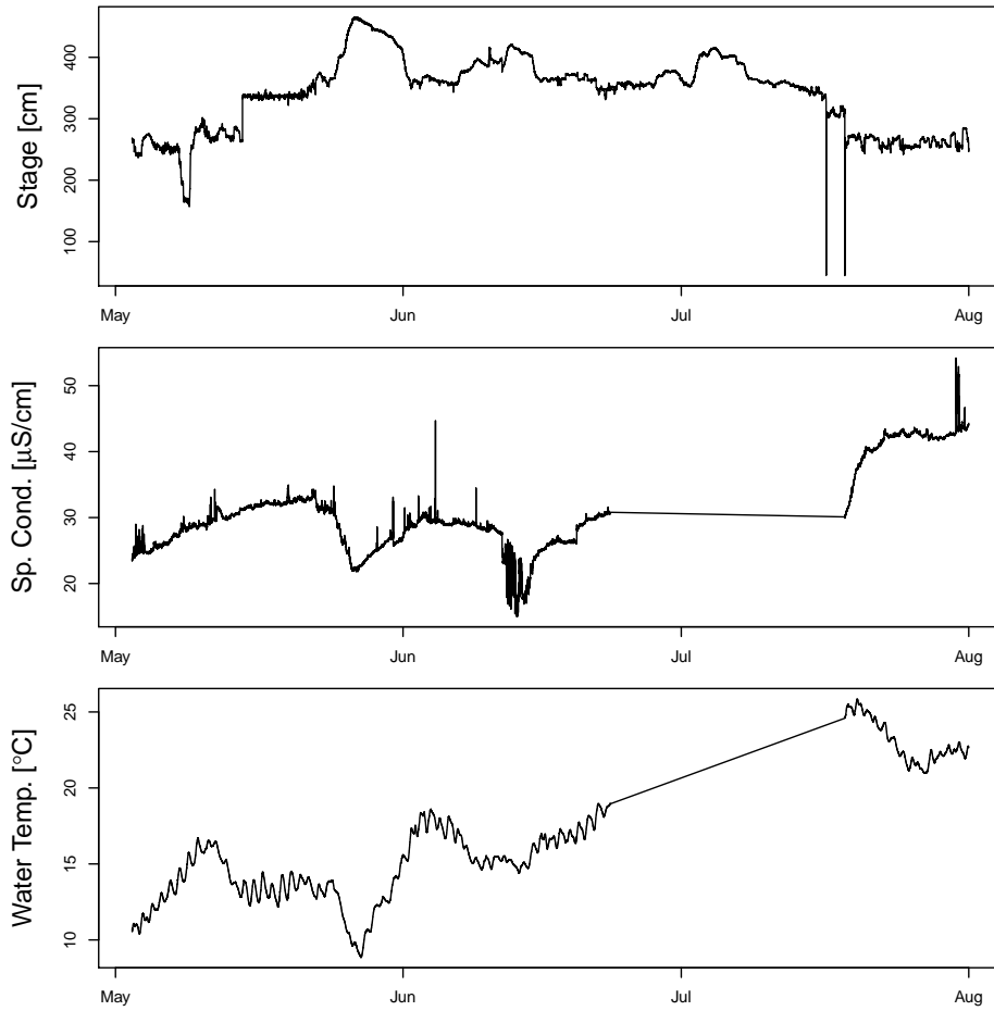
Figure 1: Stage, Specific Conductance and Water Temperature for ARD during May to July 2013
