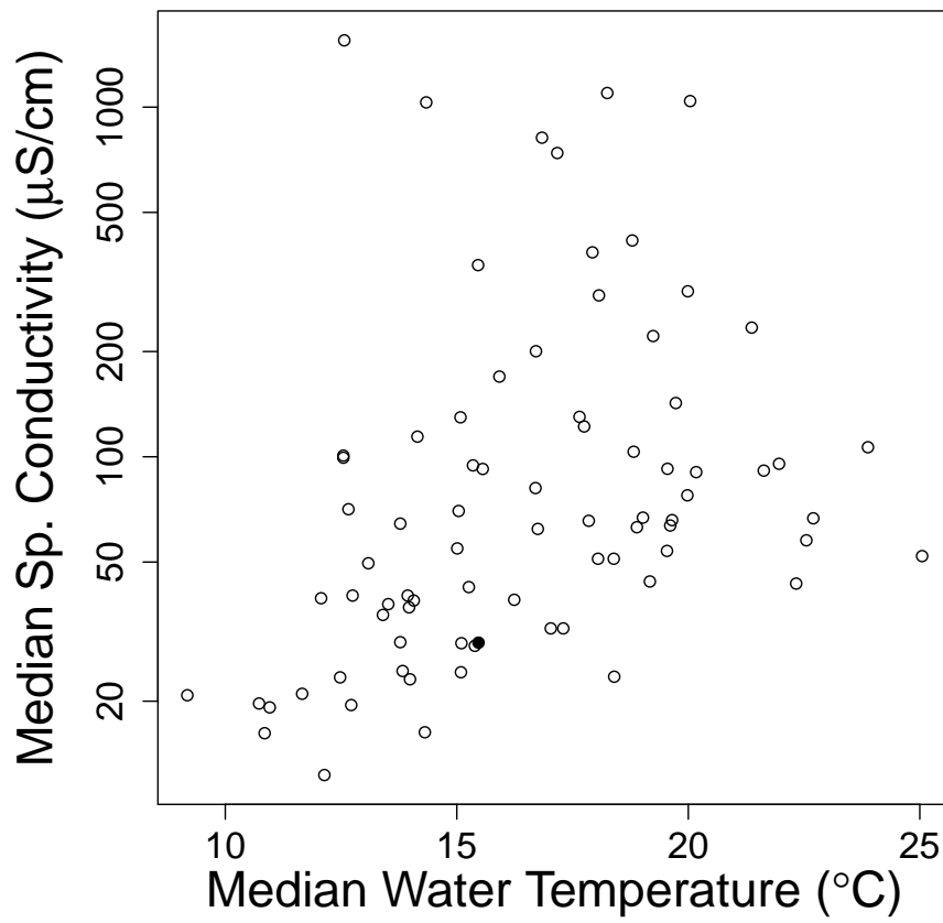
Figure 3: Median Water Temperature compared to Median Specific Conductivity for all LoVoTECS sites in New Hampshire (to date). May through July 2013. ARD is indicated as a black circle.
